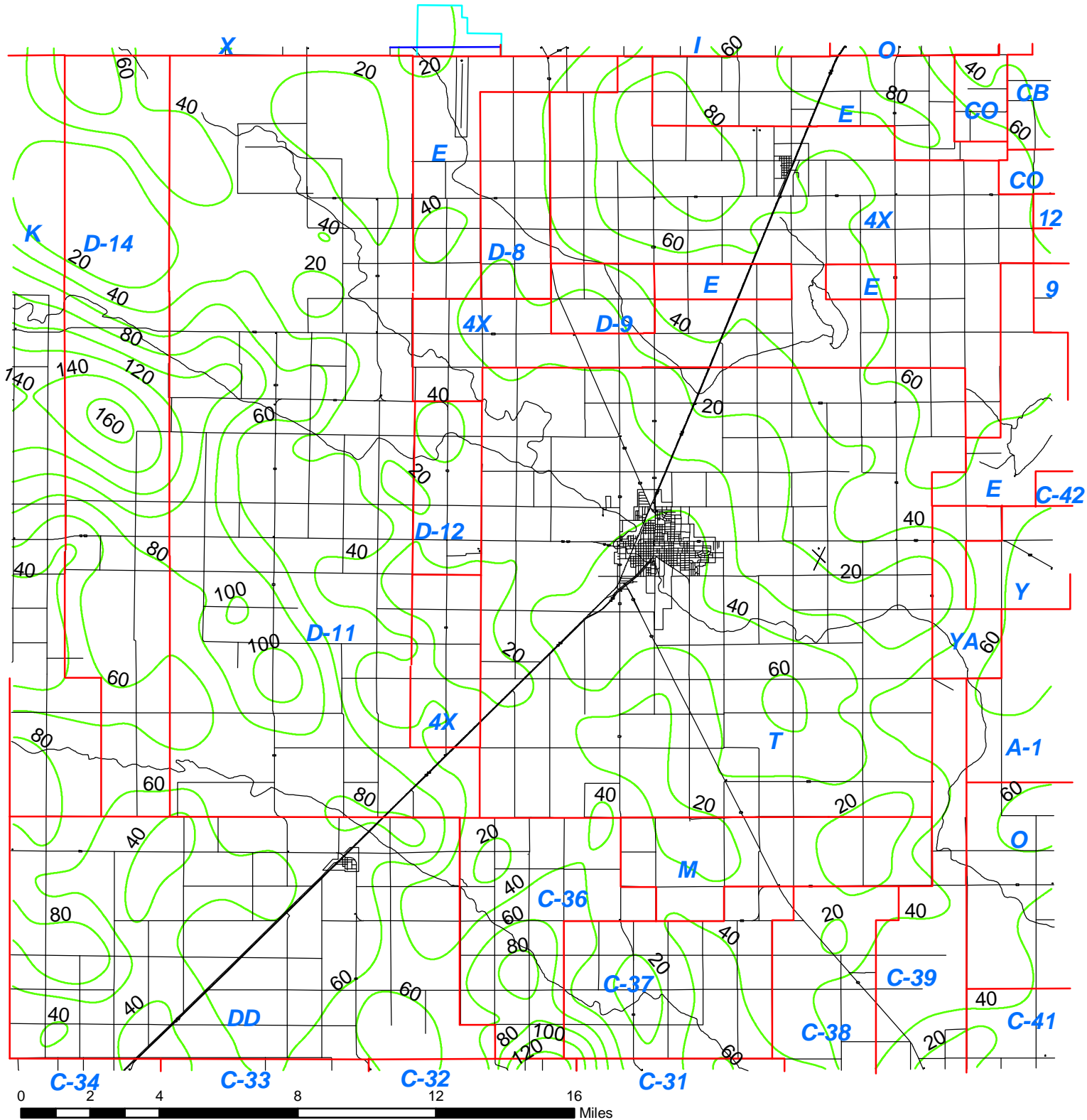
Approximate Feet of Saturated Thickness in the Ogallala Aquifer for 2005
